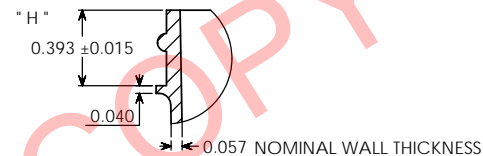
DETAIL B SCALE 2 : 1
